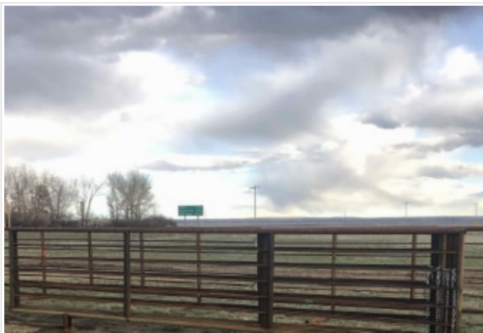
#4555C 24 foot freestanding panels 2 3/8 five bar
